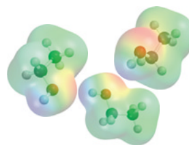
FIGURE 4.4 Hydrogen bonding in ethanol involves the oxygen of one molecule and the proton of an -OH group of another. Hydrogen bonding is much stronger than most other types of dipole-dipole attractive forces.
